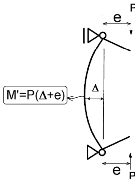
Slender column
